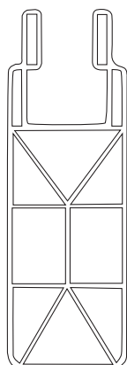
A02B 2" * 6" Enforcementfree Bottom Rail
